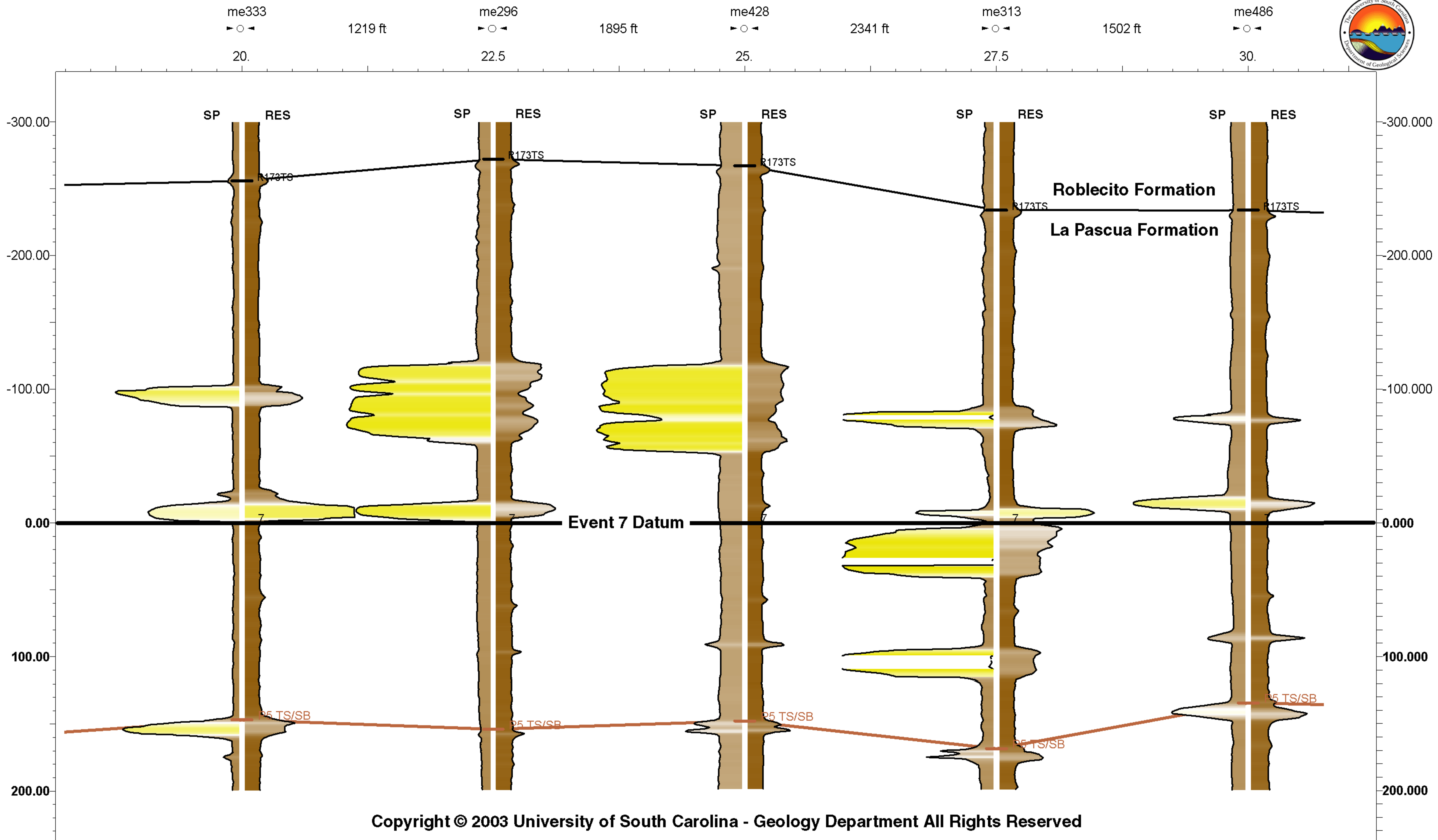
Uninterpreted Well Log Section (SP & Resitivity Logs) - 5 Wells of the Northern Strike Line, Las Mercedes Field, Guarico Sub Basin, NE Venezuela Oligocene Upper Pascua Formation (Final 3 Sequences). Flattened on "Event" 7 shale kick datum; at base is the P5 SB and at top is contact between La Pascua and Roblecito Formations (Reistroeffer 2001). Depths in feet relative to the "Event" 7 datum. Section Assembled and interpreted by P. Lake, C. G. St.C. Kendall and J. Reistroeffer - July 2003. For academic and educational puposes only.
